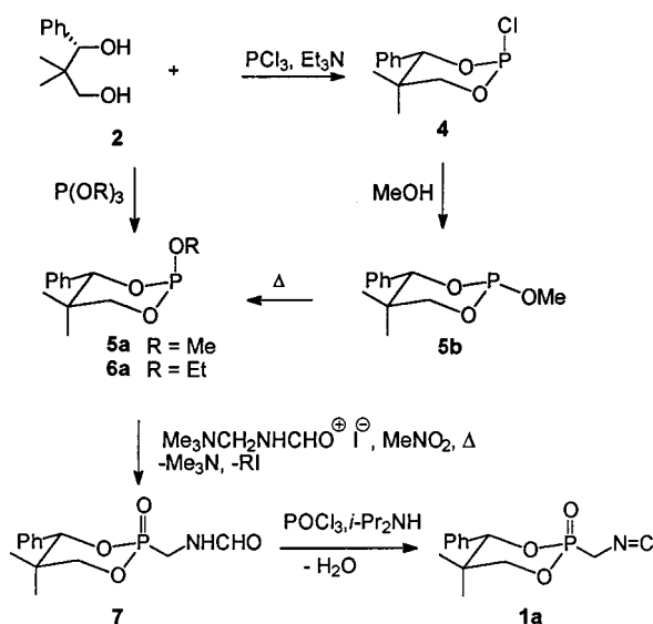
Scheme 1. Synthesis of isocyanomethylphosphorinane 1a
