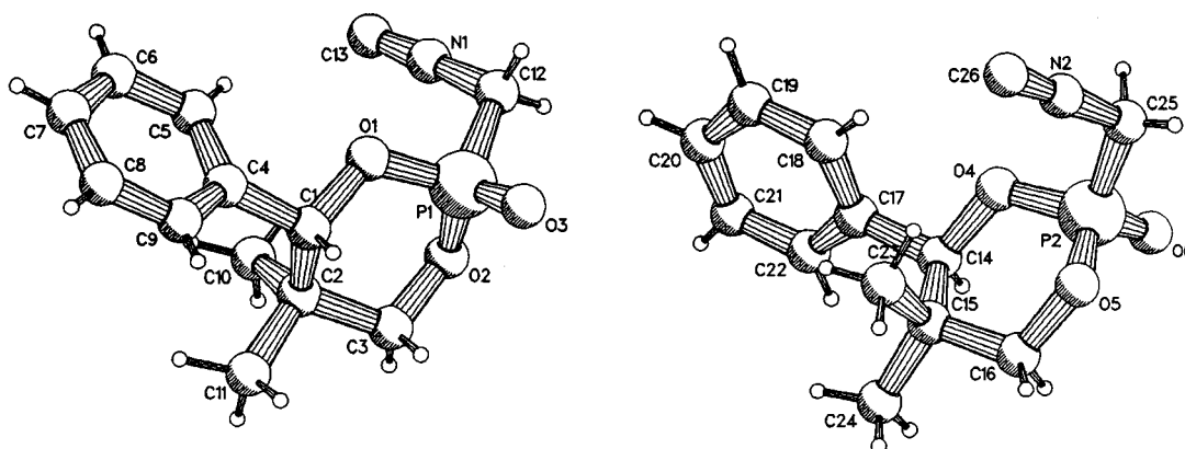
Figure 1. Single-crystal X-ray structure of ( \pm )- 1a [a]
