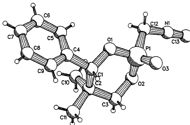
Figure 2. Single-crystal X-ray structure of (2 S ,4 S )-(–)- 1a [a]
