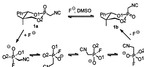
Scheme 2. Epimerization of 1a and 1b induced by \text{F}^-
